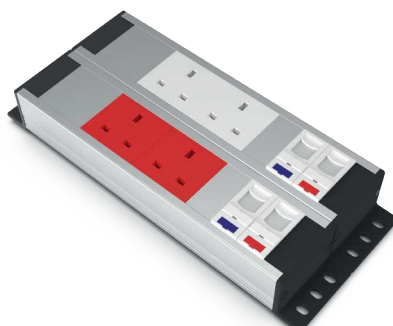
4300.4722.7822.0 2 BS Sockets + 2 BS Red Sockets + 2 Cat 6 + 2 Cat 3
